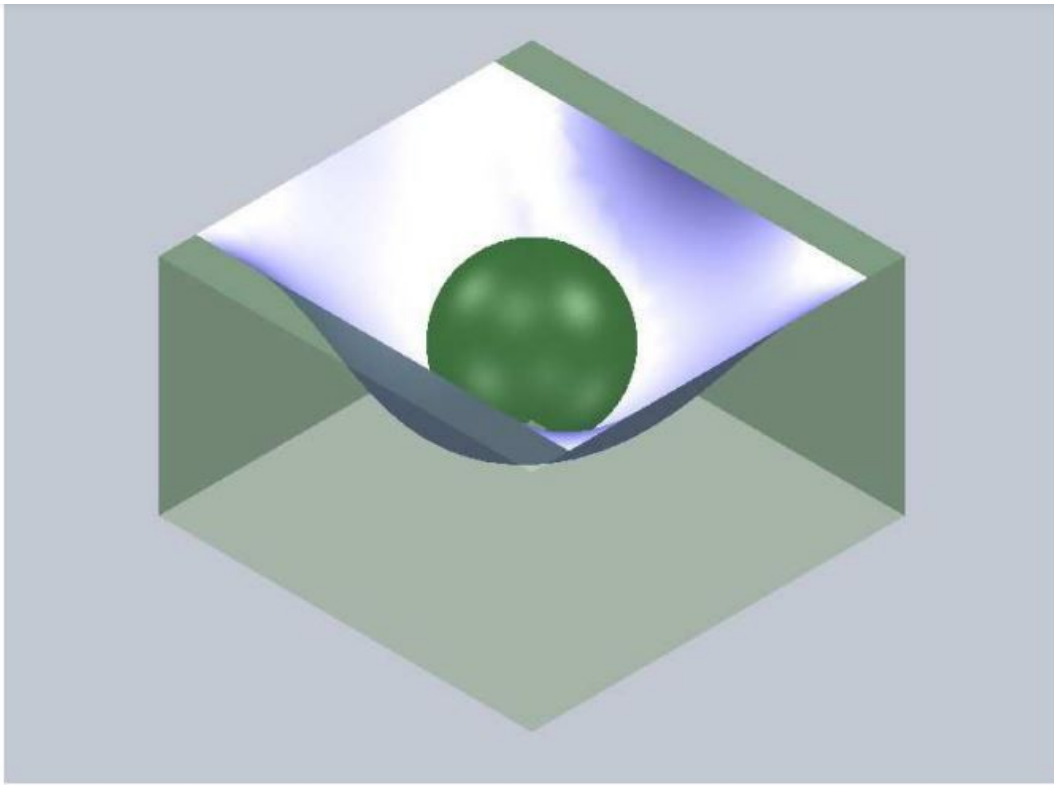
Figure 12: Earth on a dynamic space.
